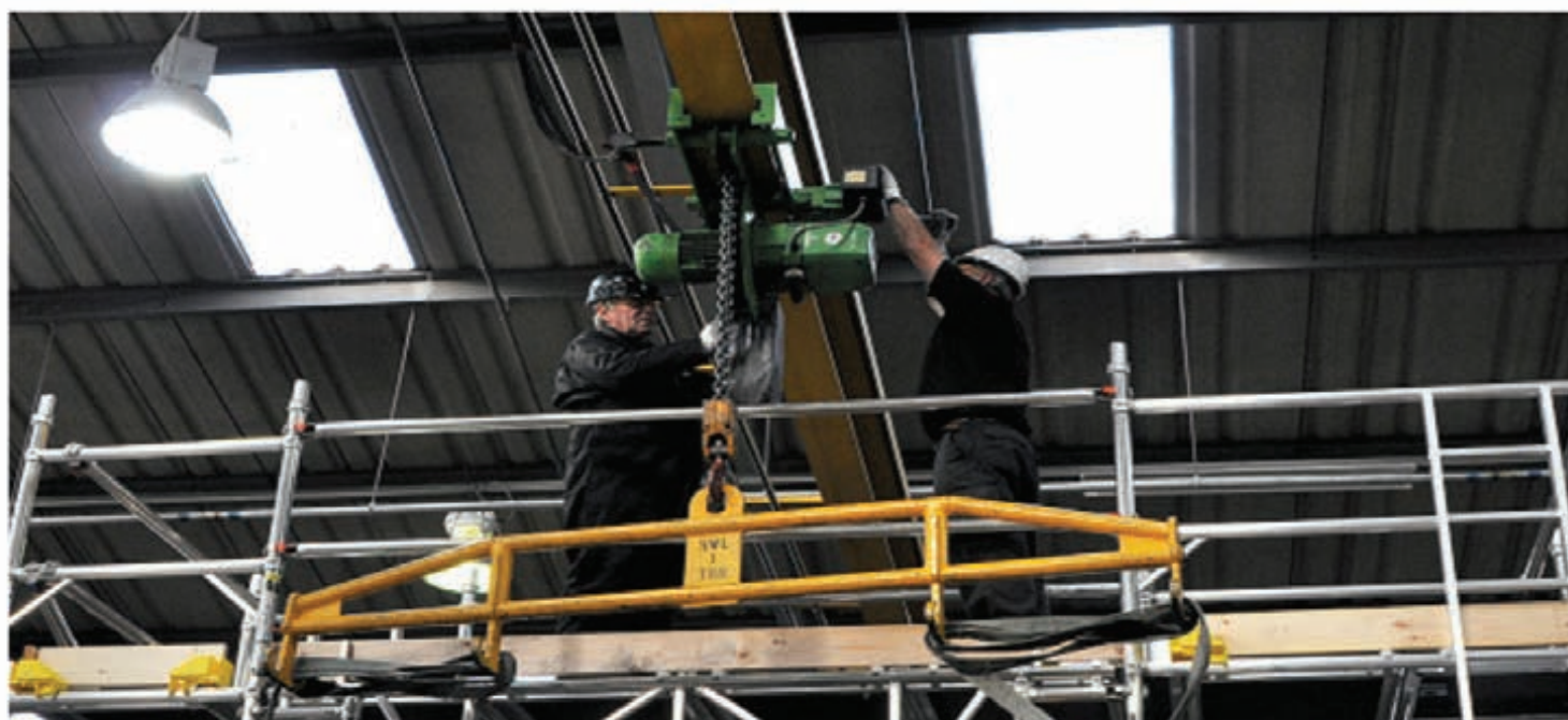
BRIDGE SYSTEM
